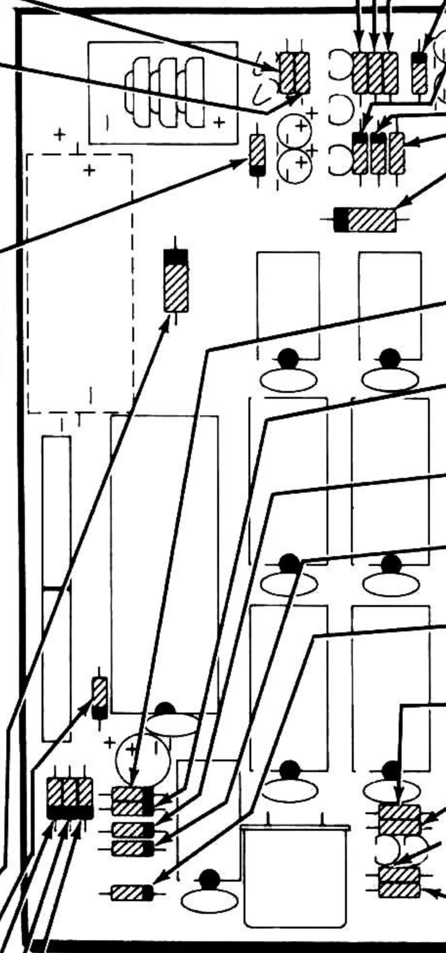
PICTORIAL 2-1
