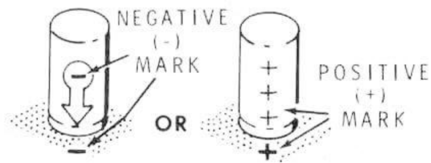
Detail 2-5A
