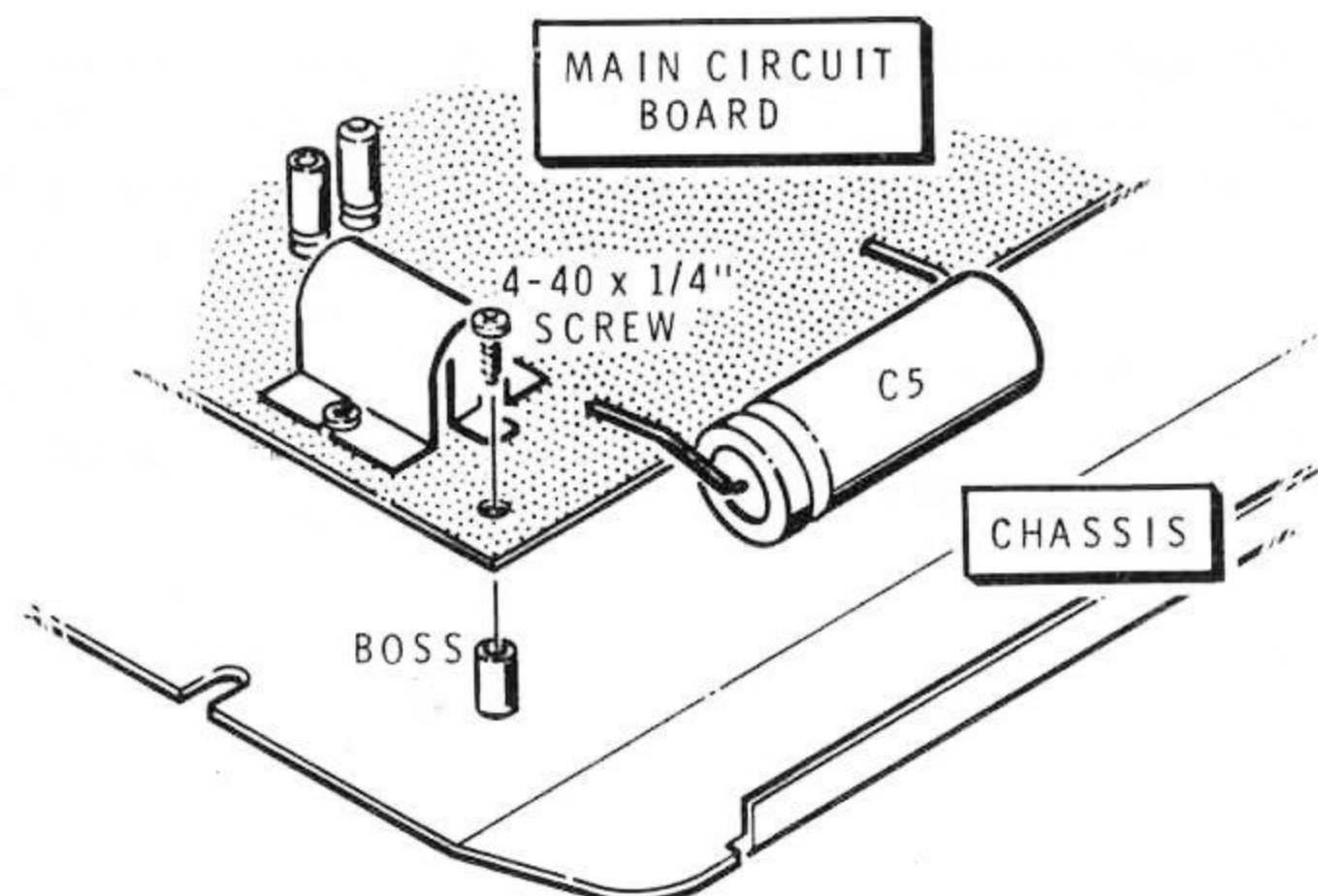
Detail 3-1N
