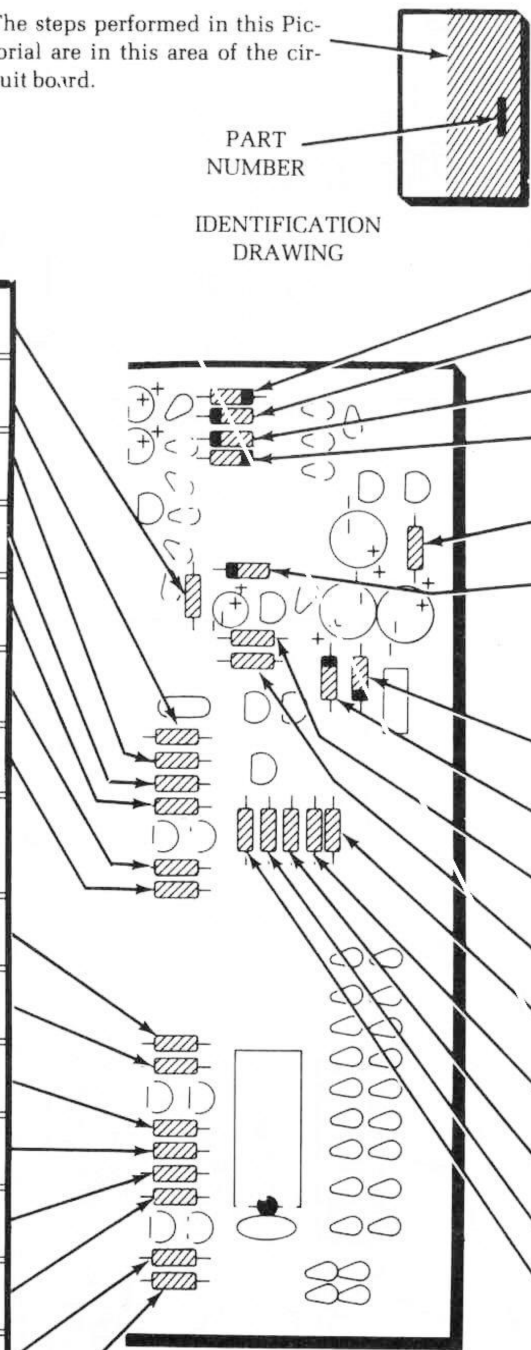
PICTORIAL 2-2
