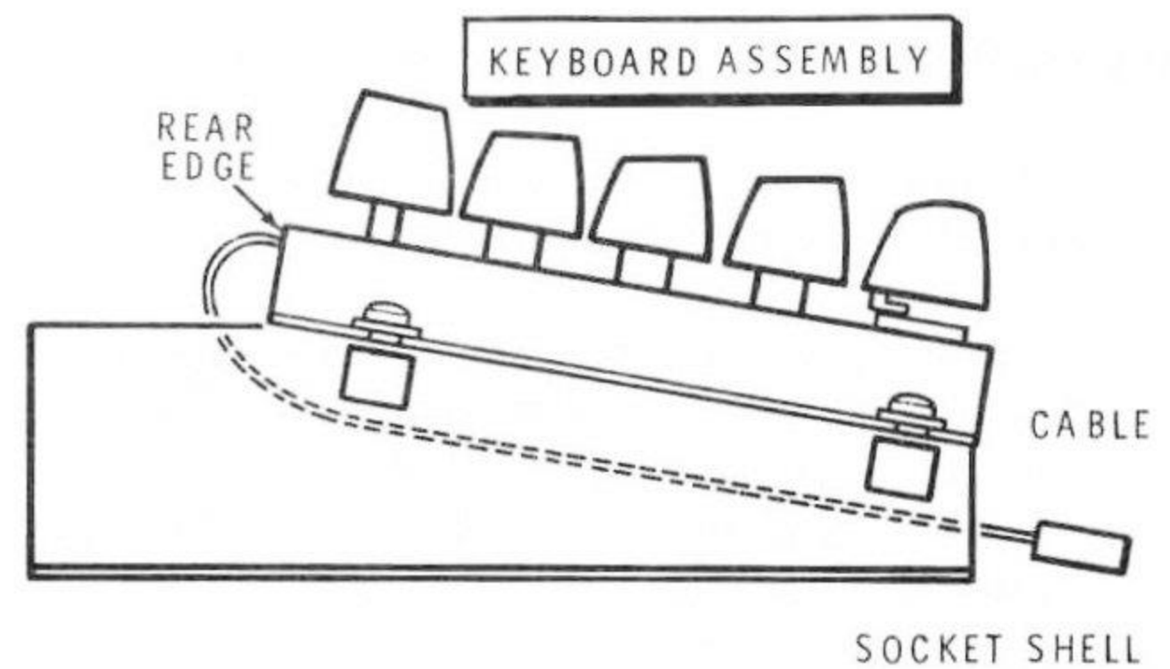
Detail 3-3C
