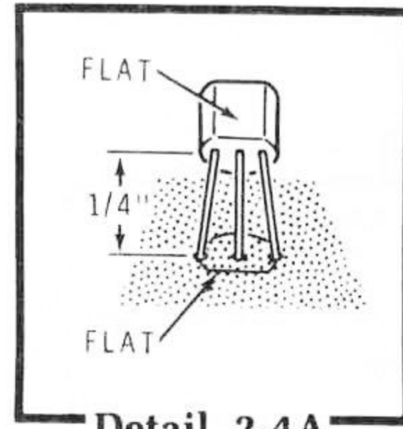
Detail 2-4A
