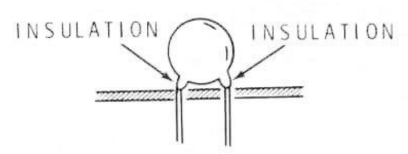
Detail 2-5B
