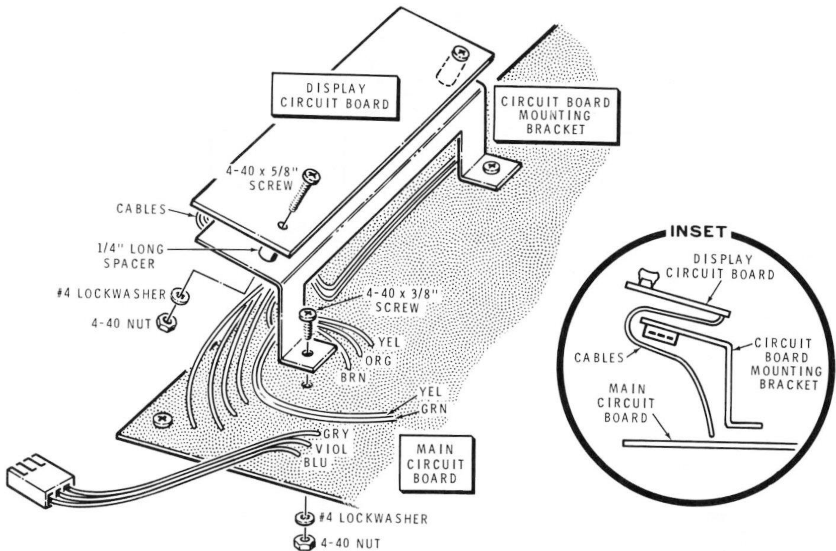
Detail 3-1K
